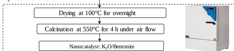
Figure 1- Preparation steps of \text{K}_2\text{O}/\text{Bentonite} Nanocatalyst via sonochemically method
