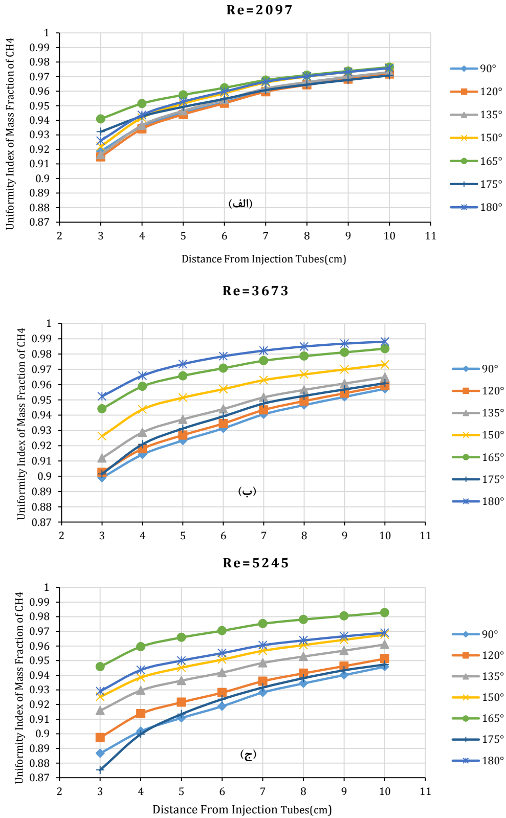
Figure 5- Uniformity Index at Cross Sections 3 to 10 cm Distant From Injection Tubes
